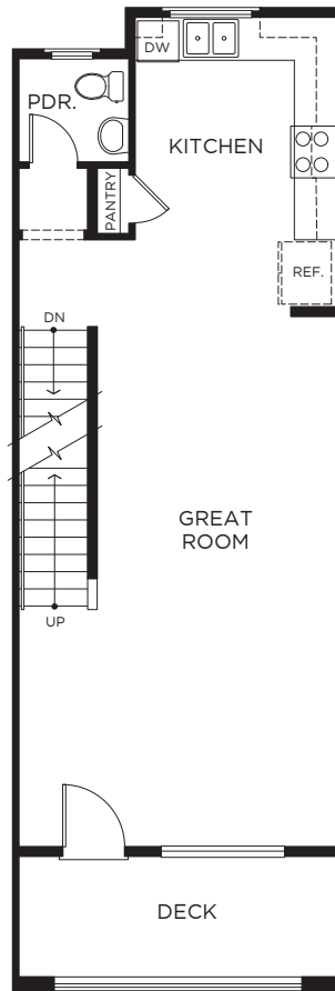
SECOND FLOOR
