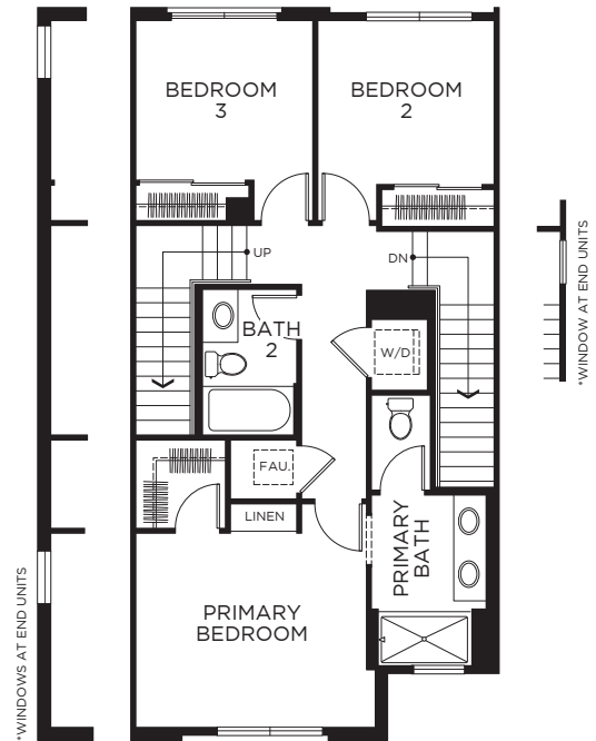
THIRD FLOOR
